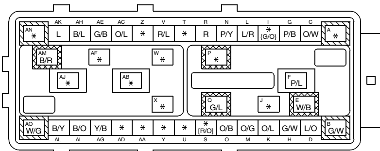
J-01 FRONT HARNESS(F)
