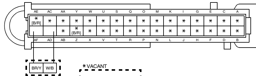
J-04 INSTRUMENT PANEL HARNESS(I)
